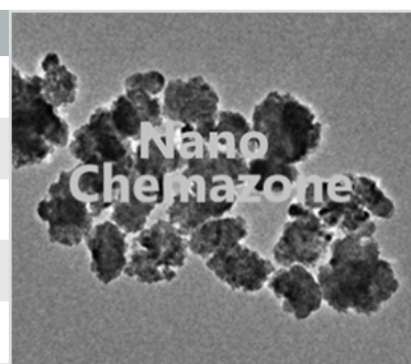
Barium Titanate
