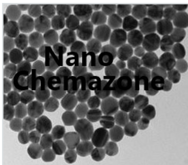
Platinum Nanoparticles
