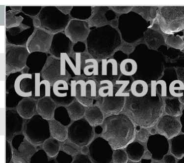
Aluminum Nanofoam
