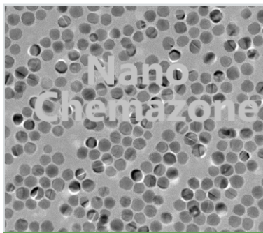
Nickel Nanoparticles
