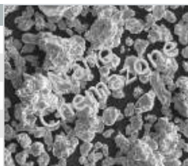
Iron Micropowder
