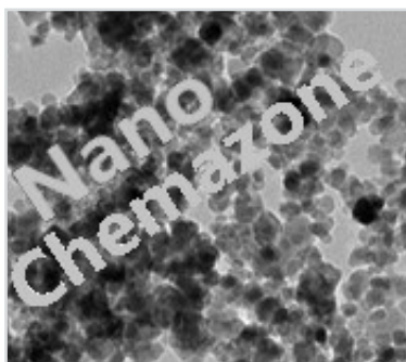
Niobium Micropowder
