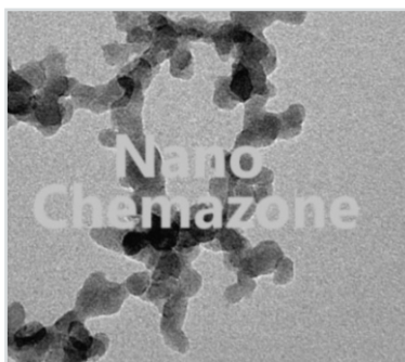
Titanium Nanoparticles
