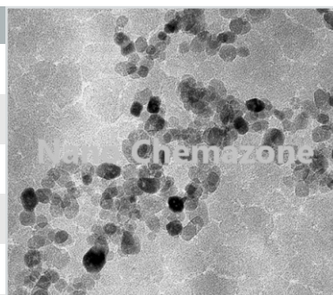
Boron Nanoparticles
