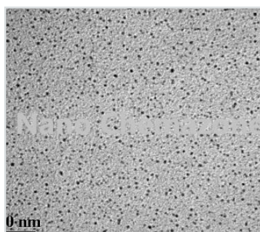
Cadmium Nanoparticles
