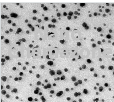
Cobalt Nanoparticles
