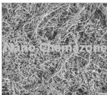
Iron Nanowires
