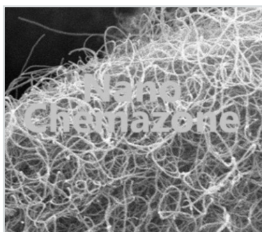
SWCNT Dispersion
