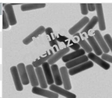
Gold Nanorods
