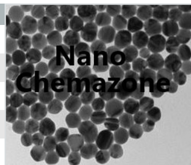
Platinum Dispersion
