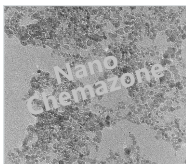
Diamond Nanoparticles
