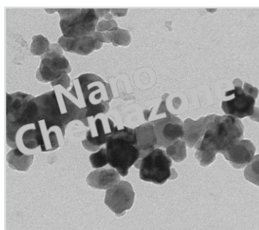
Chromium Nanoparticles
