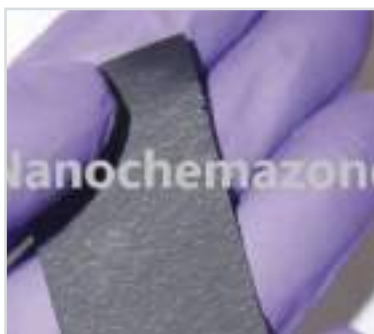
Graphdiyne Film
