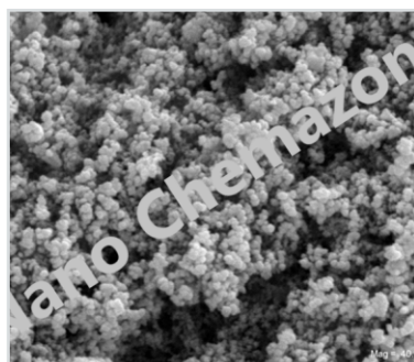
Zirconium Powder
