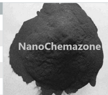
Cadmium Powder
