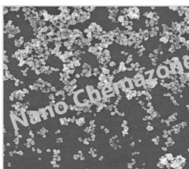
Palladium Nanopowder
