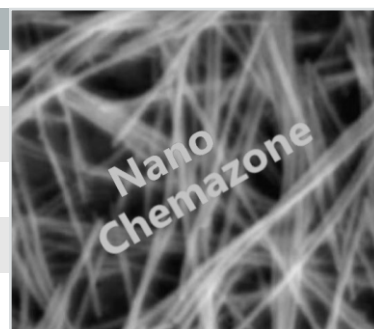
Cobalt Nanowires
