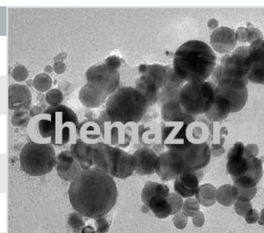
Molybdenum Nanoparticles
