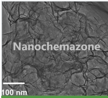
Graphdiyne Powder
